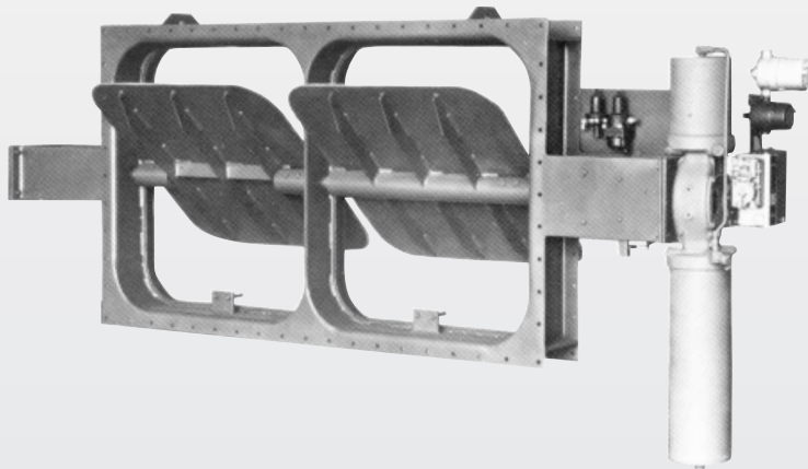
70" x 38" Type 4320 special vent isolation damper ductwork drilling, Bettis actuator with Bailey positioner.
