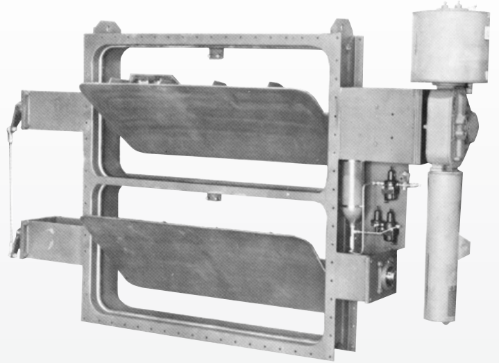
66" x 66" Type 4320 special vent isolation damper ductwork drilling Bettis actuator.
