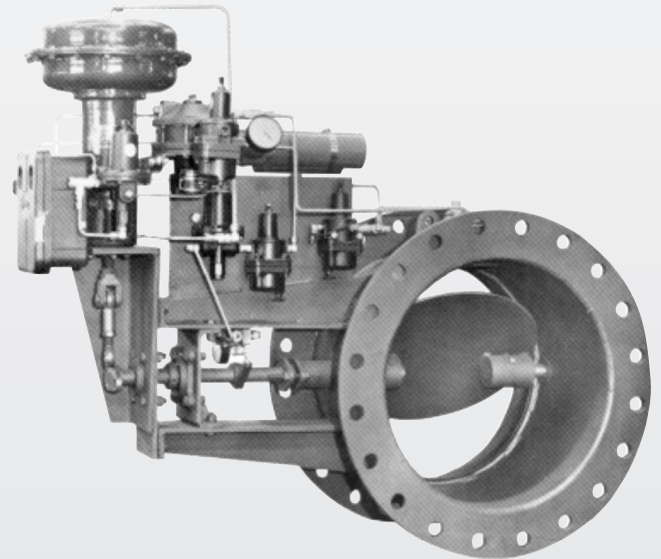
20" diameter coke oven gas isolation valve 25# AWWA drilling, Fisher 4162R controller, and Fisher 656-40 actuator and Shan-Rod seal system shown.
