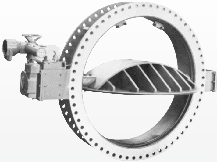
72" diameter blast furnace gas main header isolating valve 125# L.W. flanges actuator is Rotork electric.
